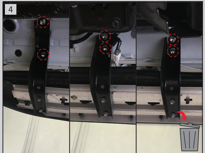
Remove 6 bolts and dispose the right step
