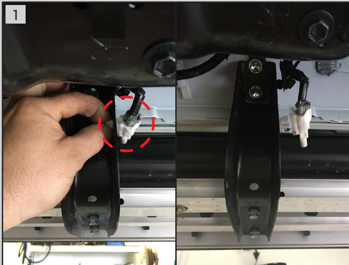
On the right step middle bracket release the electrical outlet and push it out side from the bracket
